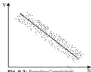
Fig. 6.2: Negative Correlation
