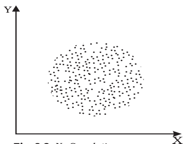
Fig. 6.3: No Correlation
